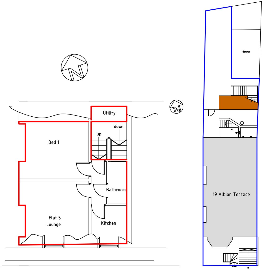
GENERAL SITE PLAN (1:200 @ A4)
